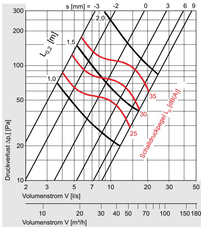
Size DN 80
