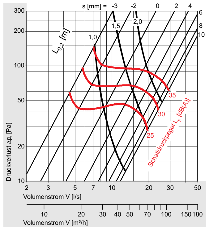
Size DN 100
