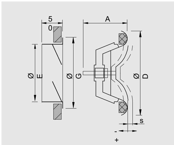
Size DN 80
