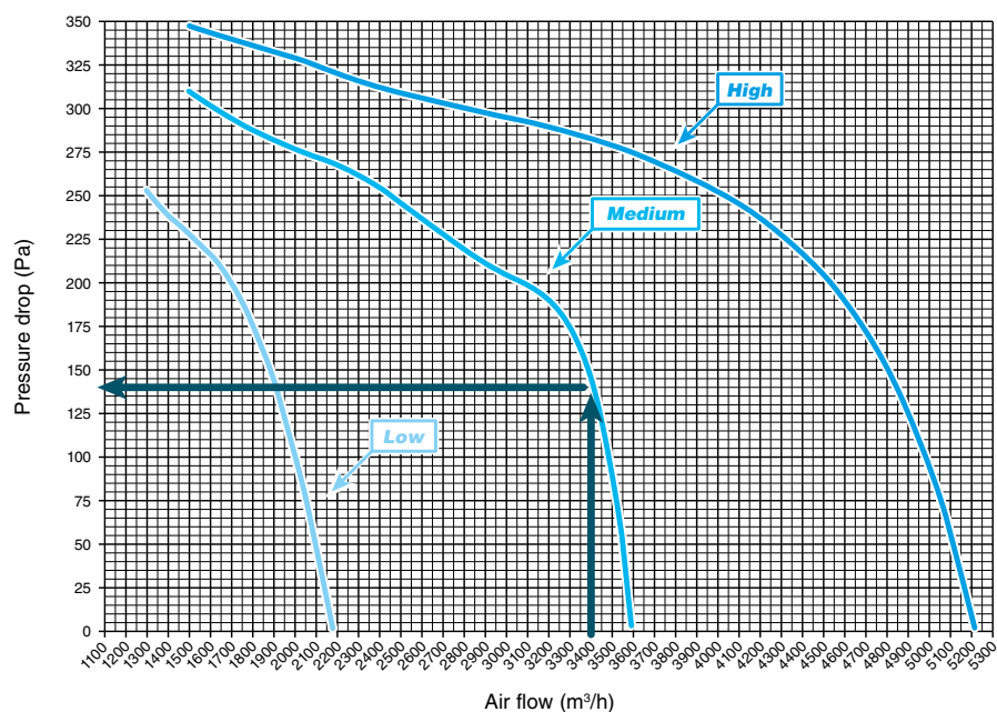
Diagram for DFCL 64 “Available pressure”
