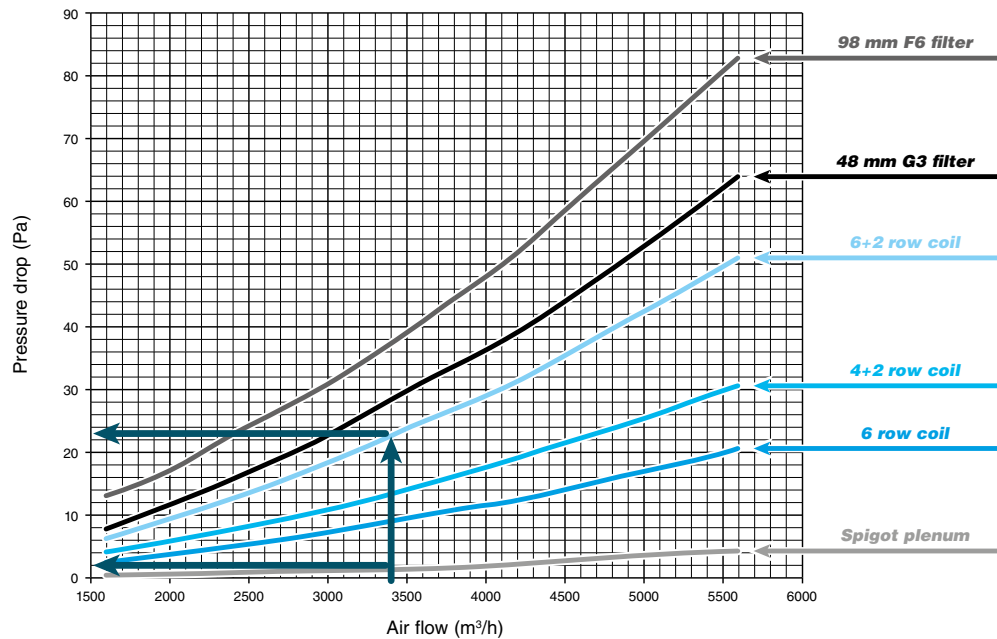
Diagram for DFCL 64 “Pressure drop”
