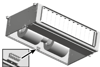
Wiring terminal board
