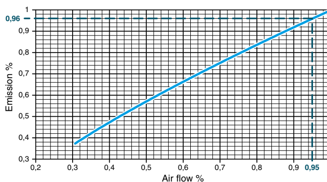
Diagram 2 – Heating emission
