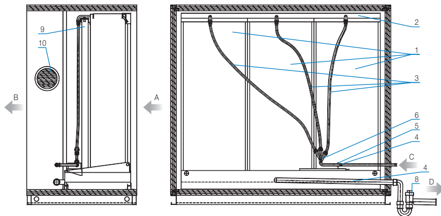
Honeycomb humidifier with direct water
