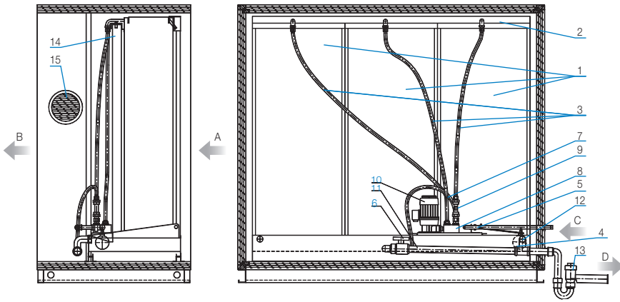
Honeycomb humidifier with circulating water
